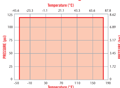
PLC Pressure Range
