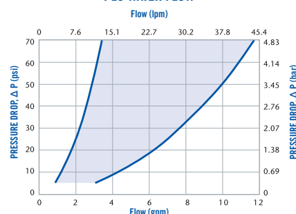
PLC WATER FLOW
